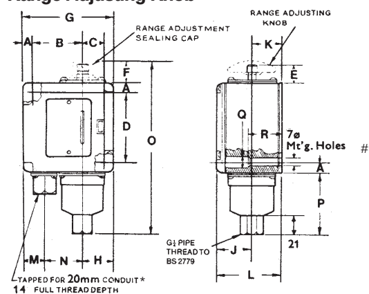
Types ACW-1, 5, 8, 9, 21, 25, 28 & 29 With Range Adjustment Sealing Cap and Range Adjusting Knob
